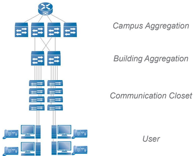
Traditional Active Ethernet LAN
